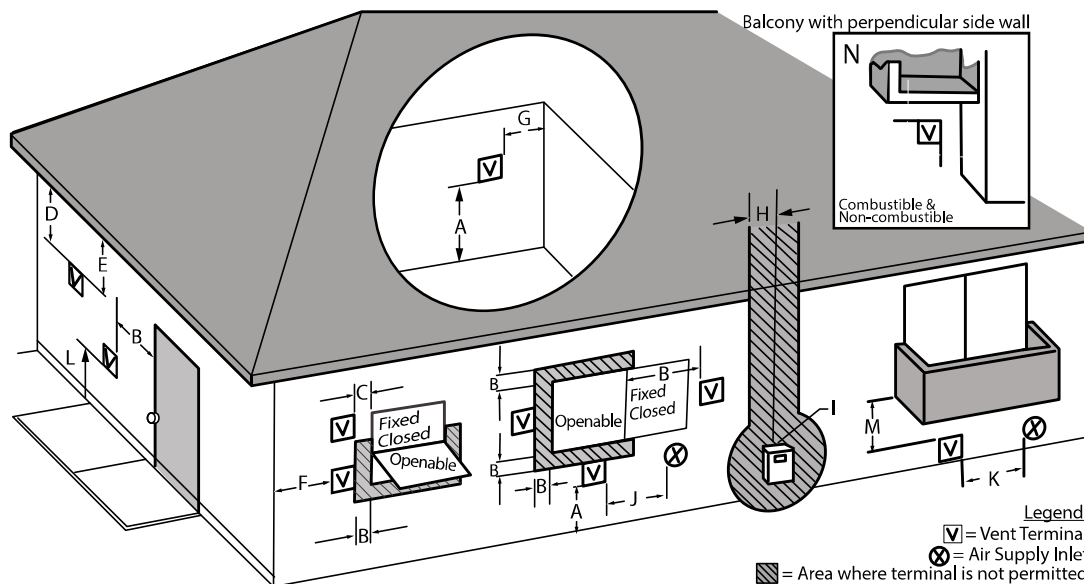
FIGURE 14B - NON-DIRECT VENT TERMINAL CLEARANCES
