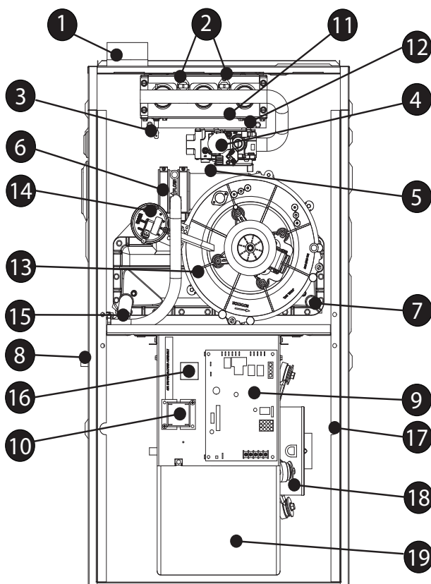
FIGURE 1 - COMPOSANTS FOURNAISE
