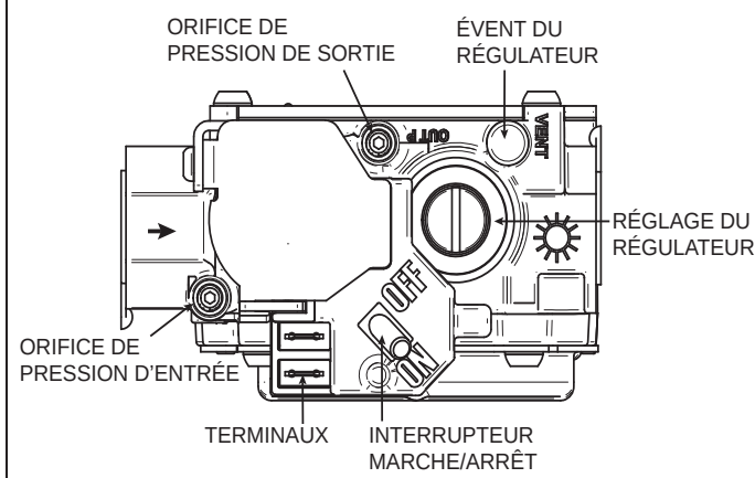
FIGURE 28 - SOUPAPE DE GAZ WHITE RODGERS 36J24-214
