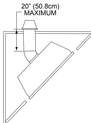
RIGID VENTING
