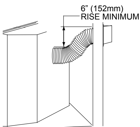
FLEXIBLE VENTING
