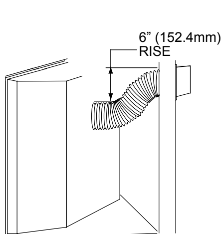
FLEX VENTING
