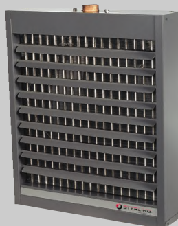
MODEL HS Header Type
